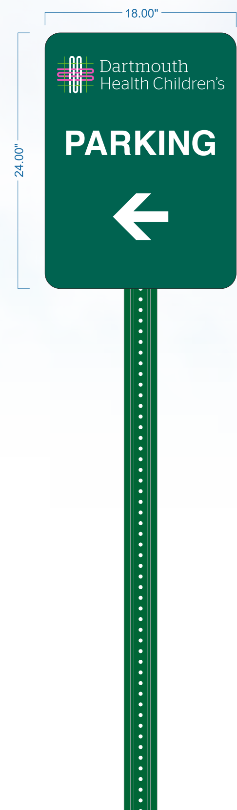
ONE (1) .080 ALUMINUM BLANK W/ APPLIED DIG. PRINT. CHANNEL POST.
