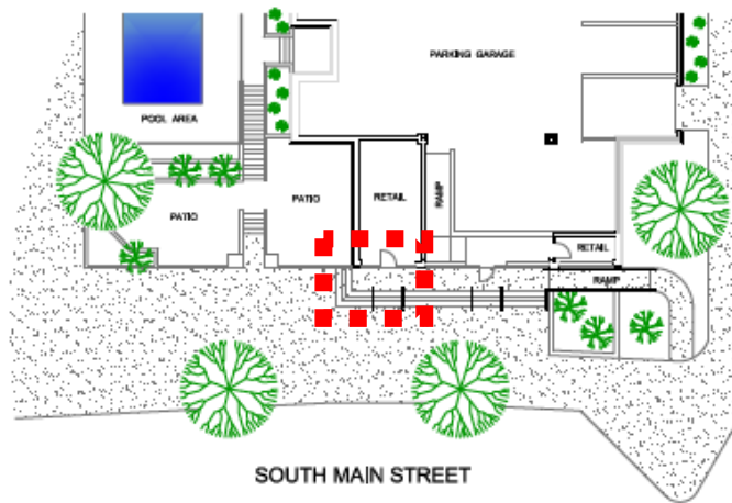
REVISED SITE PLAN (1" = 20')
