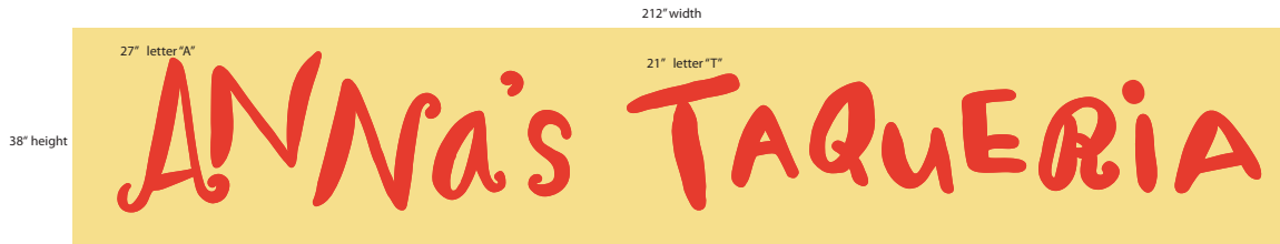
212" width 38" height 27" letter "A" 21" letter "T" 212" x 40" sign pan, painted PMS 7401 198" x 28" x 5" deep face lit letters, red can, trim, face
