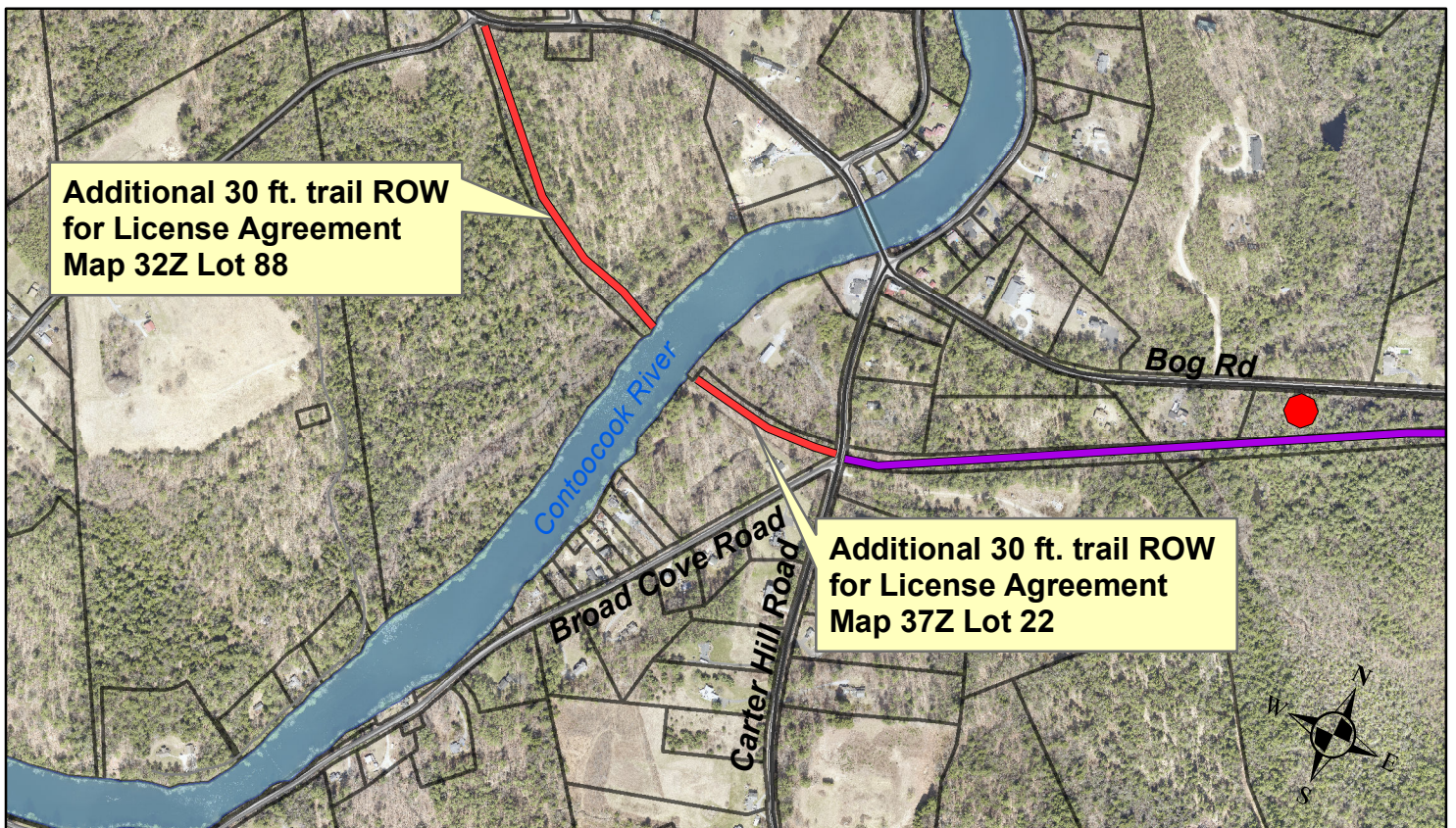
Proposed Additional Trail Right of Way Concord-Lake Sunapee Rail Trail
